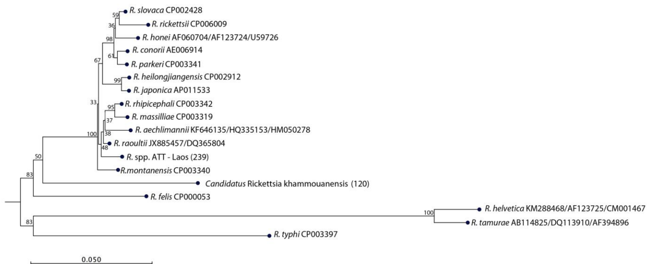
Technical Appendix Figure 4. Phylogenetic analysis of gltA , 17 kDa, and ompB genes of Rickettsia spp., Kammouan Province, Laos. The tree was constructed by using partial nucleotide sequences (1,114–1,117 bp) of concatenated sequences of gltA , 17-kDa, and ompB genes; the Kimura-80 model; and the neighbor-joining method. Analyses were supported by using bootstrap analysis with 1,000 replications. Numbers along branches are bootstrap values. Sample numbers identifying each tick pool from this study are shown in parentheses after the sequence name. Scale bar indicates nucleotide substitutions per site.
