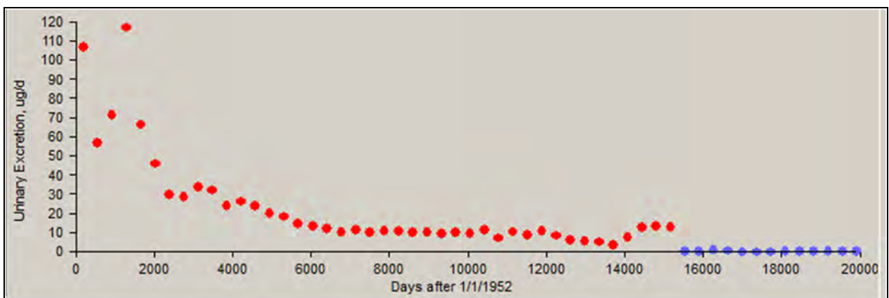
Figure A-4. Predicted values (line) versus measured results (blue dots), 01/01/1994 to 12/31/2006, 84th percentile, type F.
