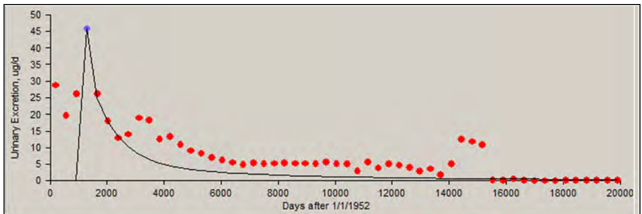
Figure A-10. Predicted values (line) versus measured results (blue dots), 01/01/1955 to 12/31/1955, 50th percentile, type S.
