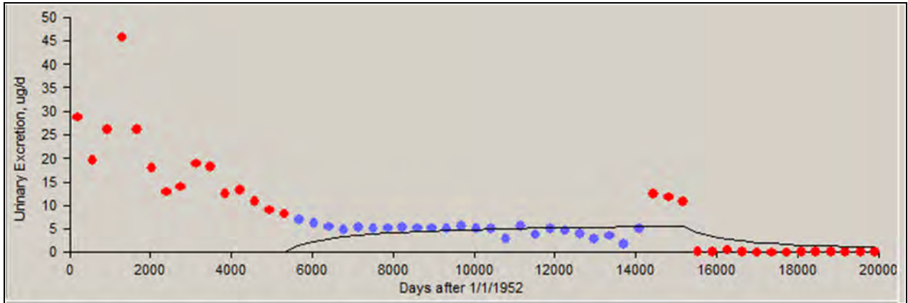
Figure A-14. Predicted values (line) versus measured results (blue dots), 01/01/1967 to 12/31/1993, 50th percentile, type S.
