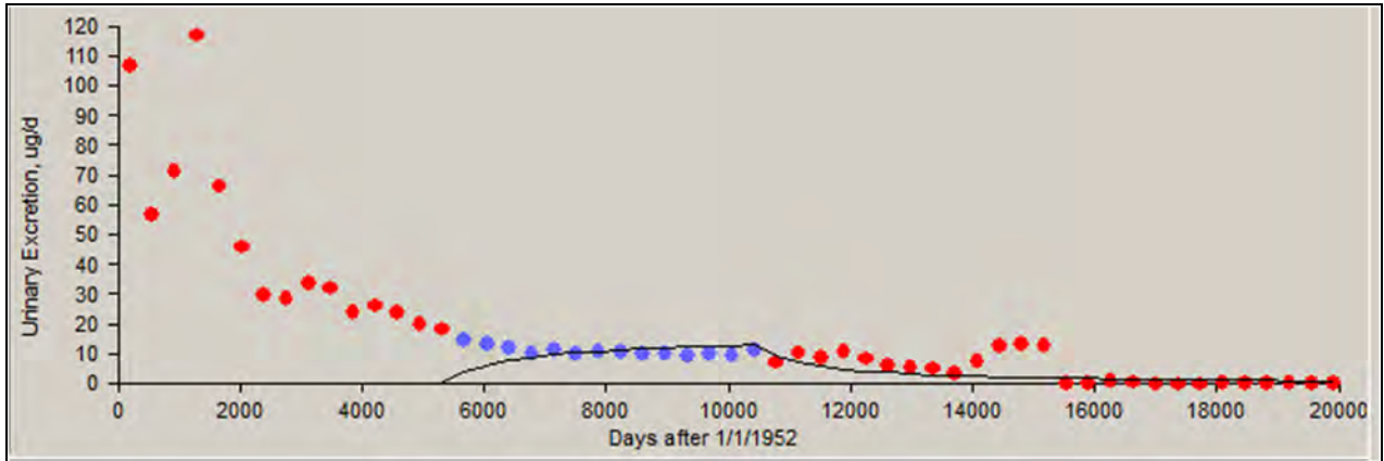
Figure A-20. Predicted values (line) versus measured results (blue dots), 01/01/1967 to 12/31/1980, 84th percentile, type S.
