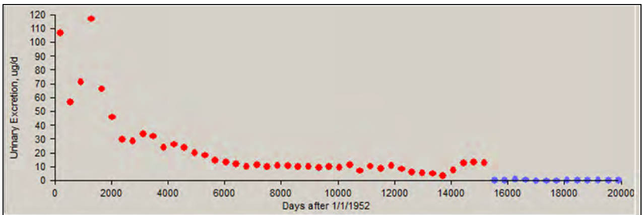
Figure A-22. Predicted values (line) versus measured results (blue dots), 01/01/1994 to 12/31/2006, 84th percentile, type S.
