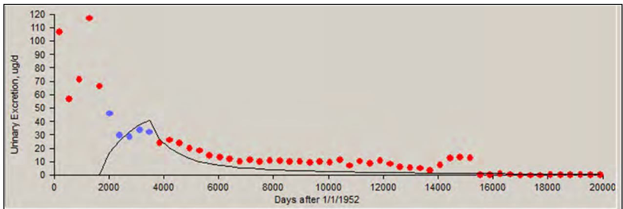
Figure A-18. Predicted values (line) versus measured results (blue dots), 01/01/1957 to 12/31/1961, 84th percentile, type S.
