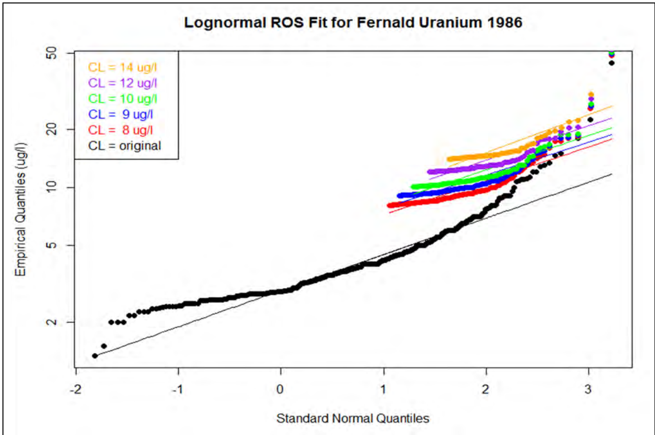
Figure 2-1. Change in lognormal fit for various CLs.
