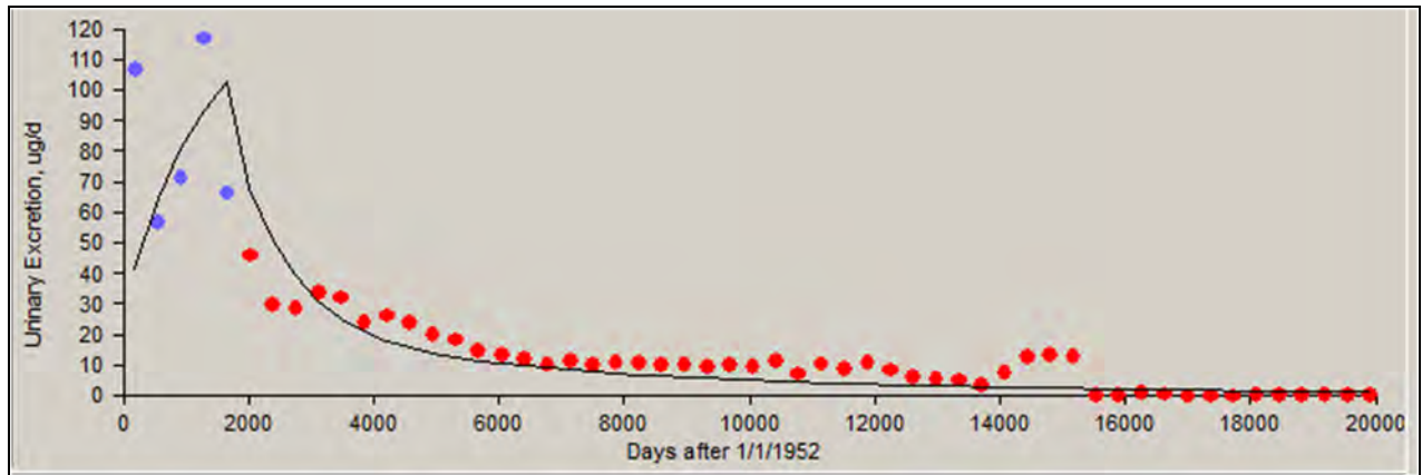
Figure A-17. Predicted values (line) versus measured results (blue dots), 01/01/1952 to 12/31/1956, 84th percentile, type S.
