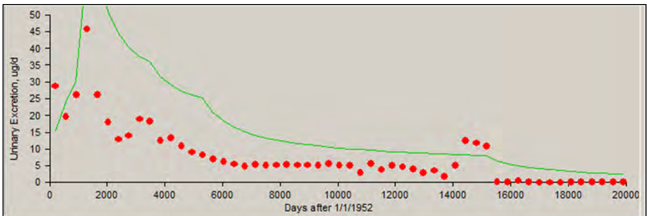
Figure A-16. Summarized results of the predicted values (line) versus the excluded results (red dots), 01/01/1952 to 12/31/2006, 50th percentile, type S.
