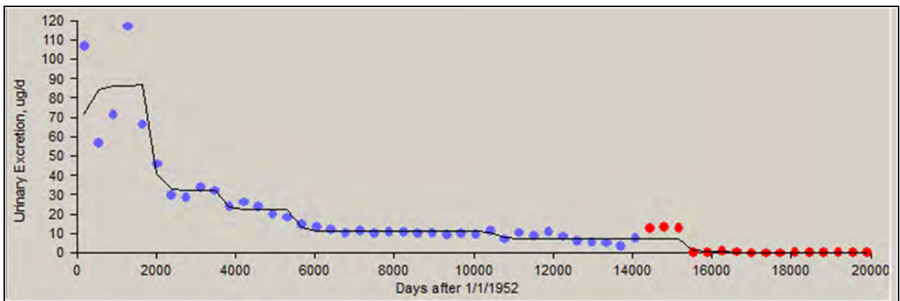
Figure A-7. Predicted values (line) versus measured results (blue dots), 01/01/1952 to 12/31/1993, 84th percentile, type M.
