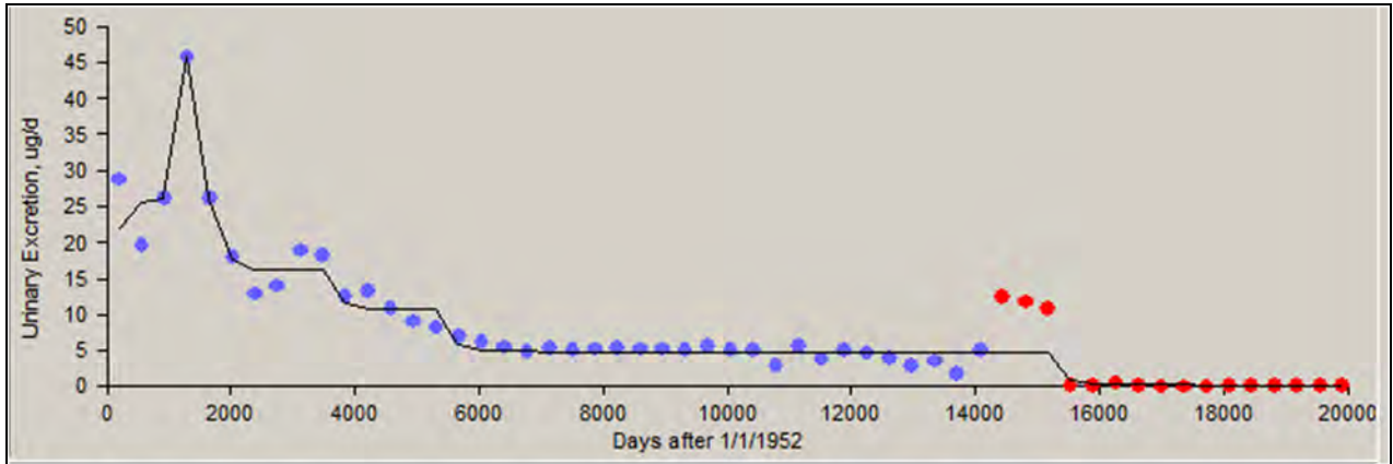
Figure A-5. Predicted values (line) versus measured results (blue dots), 01/01/1952 to 12/31/1993, 50th percentile, type M.
