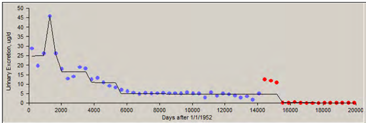
Figure A-1. Predicted values (line) versus measured results (blue dots), 01/01/1952 to 12/31/1993, 50th percentile, type F.
