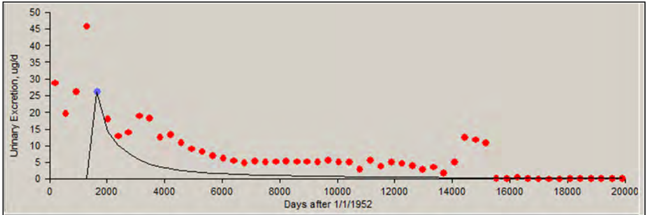
Figure A-11. Predicted values (line) versus measured results (blue dots), 01/01/1956 to 12/31/1956, 50th percentile, type S.
