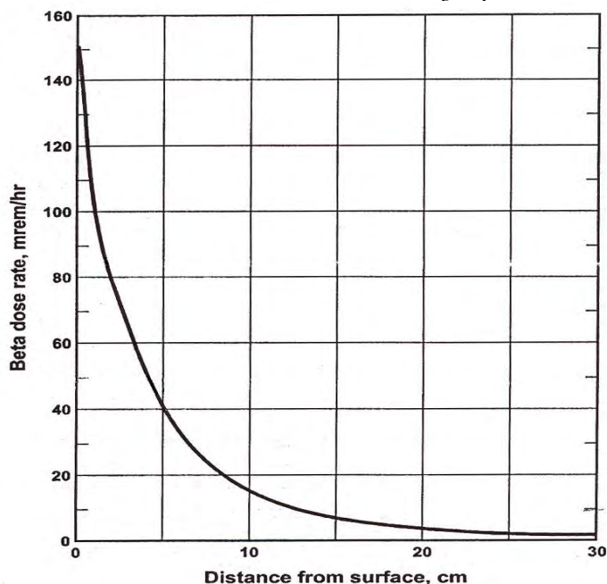
Figure 1: Beta dose rate from yellowcake separated from ore for more than 100 days as a function of distance from the surface. [Reproduced from US NRC 2002a]
