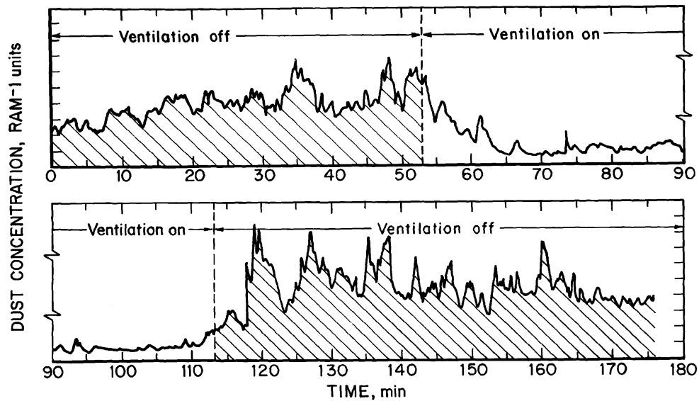
Figure 3.—Respirable dust levels at location 5 with and without total mill ventilation system.
