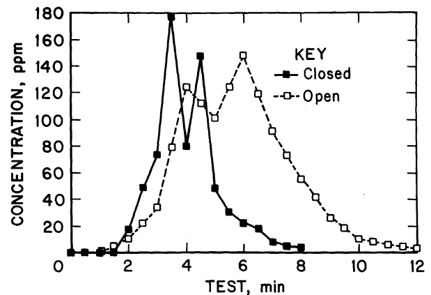
Figure 10. -SF 6 analysis-effectiveness of total mill ventilation system with windows open versus closed. Concentrations recorded at east fan.
