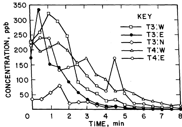
Figure 9. -SF 6 analysis-comparing four fans (T3) versus two fans (T4) for total mill ventilation system. W, concentration recorded at west fan; E, concentration measured at east fan
