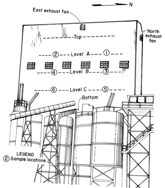
Figure 5.- Six dust monitoring locations at mill 2.
