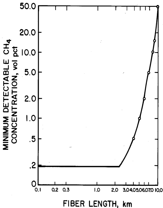
Figure 5.—Minimum detectable CH 4 concentration as function of fiber length.
