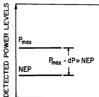
Figure 7.—Long-range limitation. (NEP = noise equivalent power of detector; dP = fractional drop in received power when CH 4 is introduced into gas cell; P max = power received at detector for a given length of fiber with no CH 4 present.)
