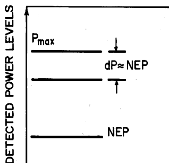
Figure 6.—Short-range limitation. (NEP = noise equivalent power of detector; dP = fractional drop in received power when CH 4 is introduced into gas cell; P max = power received at detector for a given length of fiber with no CH 4 present.)
