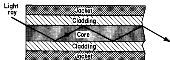
Figure 1.—Profile of fiber-optic cable.
