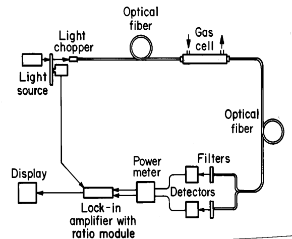
Figure 2.—Fiber-optic CH 4 monitor.
