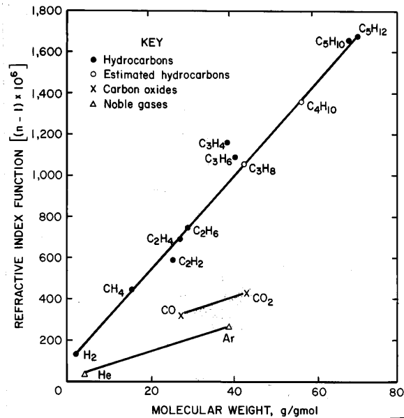
Figure 8.—Refractive index as function of molecular weight.
