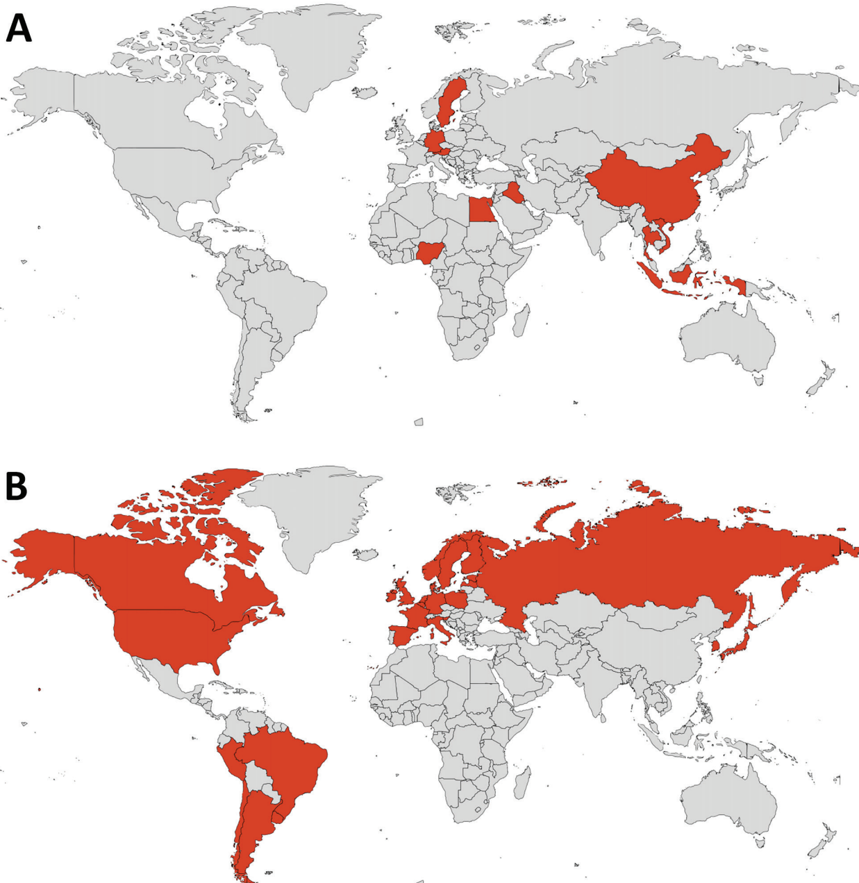
Figure 1. Geographic location of mammal species affected by highly pathogenic influenza virus A(H5N1) in previous waves of infection, 2003–2019 (A), and in the current panzootic, 2020–2023 (B).
