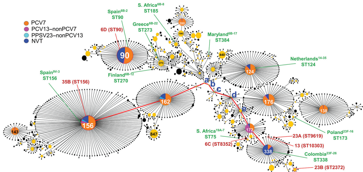
Figure 4. Details of Streptococcus pneumoniae clonal complex (CC) 156 (n = 4,736), including 1,308 sequence types obtained from the multilocus sequence typing website ( https://pubmlst.org/spneumoniae/ ). Data include those from this study (n = 359). STs of 6 genotypes for penicillin-resistant S. pneumoniae identified in NVT serotypes belonged to CC156. STs of serotypes 6C, 13, 23A, and 23B were derived from ST338 and ST172 (shown in red). Serotypes 6D and 35B belonged to ST90 and ST156, respectively. The Pneumococcal Molecular Epidemiology Network clone identified in CC156 is also shown (in green). The red line indicates evolution from ST156 to ST338: a, ST8055; b, ST8618; c, ST4542; d, ST171; e, ST361. NVT, nonvaccine serotype; PCV7, 7-valent pneumococcal conjugate vaccine; PCV13, 13-valent pneumococcal conjugate vaccine; PPSV23, 23-valent pneumococcal polysaccharide vaccine; ST, sequence type.
