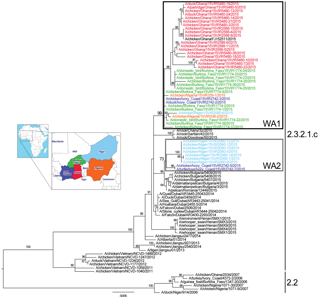
Figure. Maximum-likelihood phylogenetic tree of the hemagglutinin gene segment of highly pathogenic avian influenza (H5N1) viruses from West Africa. Strain colors indicate country of collection (inset). The 2 identified groups (WA1 and WA2) are indicated by boxes (black and gray, respectively). Clades are indicated at right; sequences from the 2006–2008 epidemic (clade 2.2) in West Africa were used as an outgroup. Numbers at the nodes represent bootstrap values >60%, obtained through a nonparametric bootstrap analysis that used 100 replicates. Scale bar indicates nucleotide substitutions per site.
